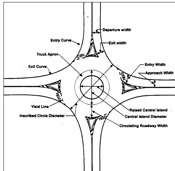
Figure 4.15. Standard Roundabout Design Used in Florida.
