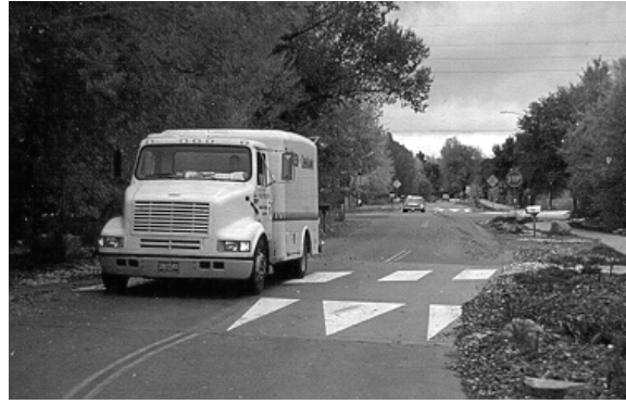
Figure 7.16. 46-foot (12 foot, 22 foot, 12 foot) Raised Crosswalk. (Boulder, CO)
