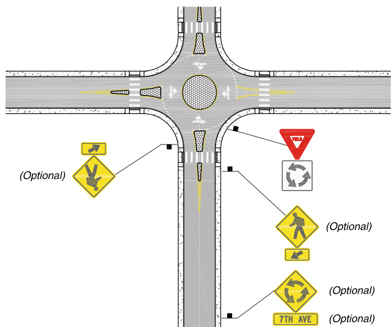
Figure 7: Sample Signing Plan for a Mini-Roundabout
